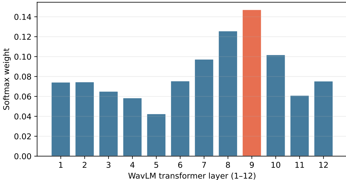
Learned layer fusion (peak: Layer 9, entropy=2.43)
