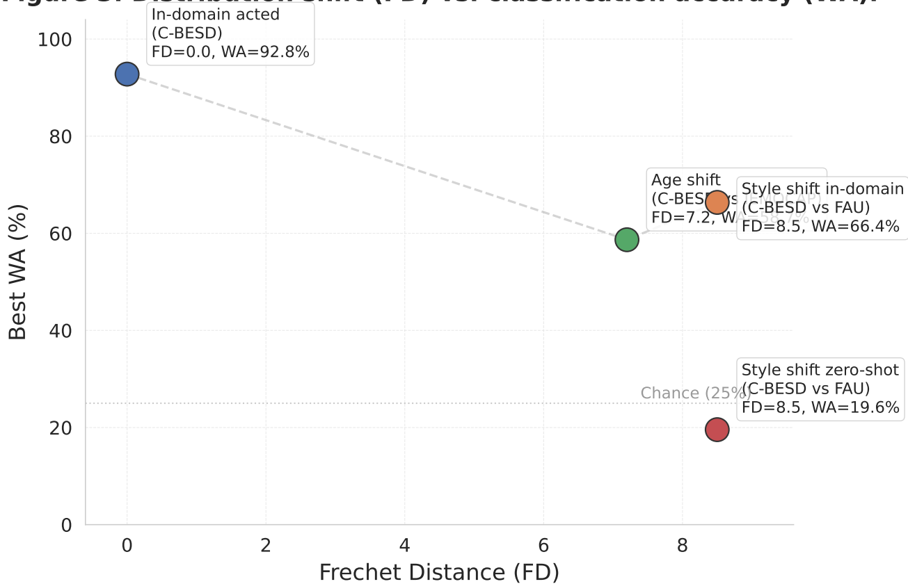
Figure 3: Distribution shift (FD) vs. classification accuracy (WA).
