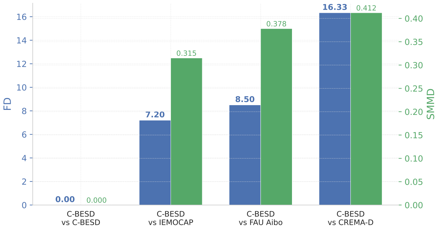
Figure 4: Cross-corpus distribution shift diagnostics (FD and SMMD).
