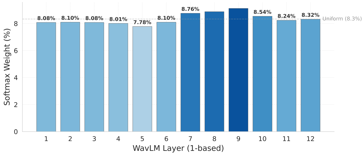
Figure 5: Learned softmax weights over WavLM layers 1-12 (peak at Layer 9).
