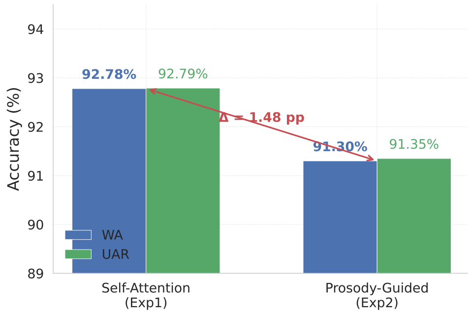
Figure 6: C-BESD acted corpus: self-attention vs prosody-guided pooling.
