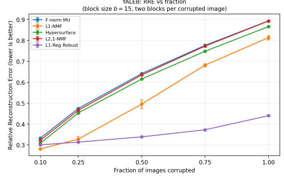
(b) Extended YaleB
