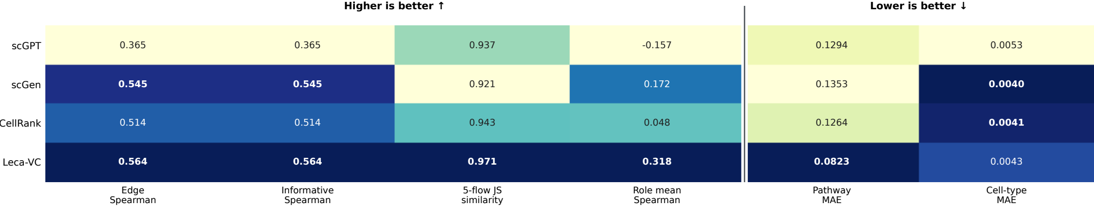
A. CCI reconstruction accuracy
