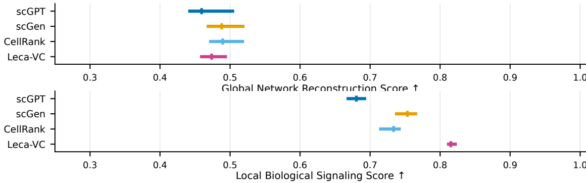
B. Network and biological signaling reconstruction stability
