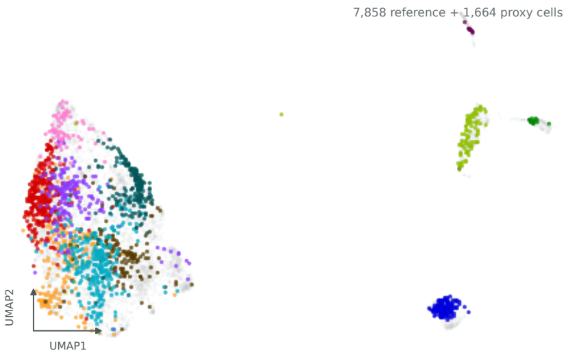
C. WOT
