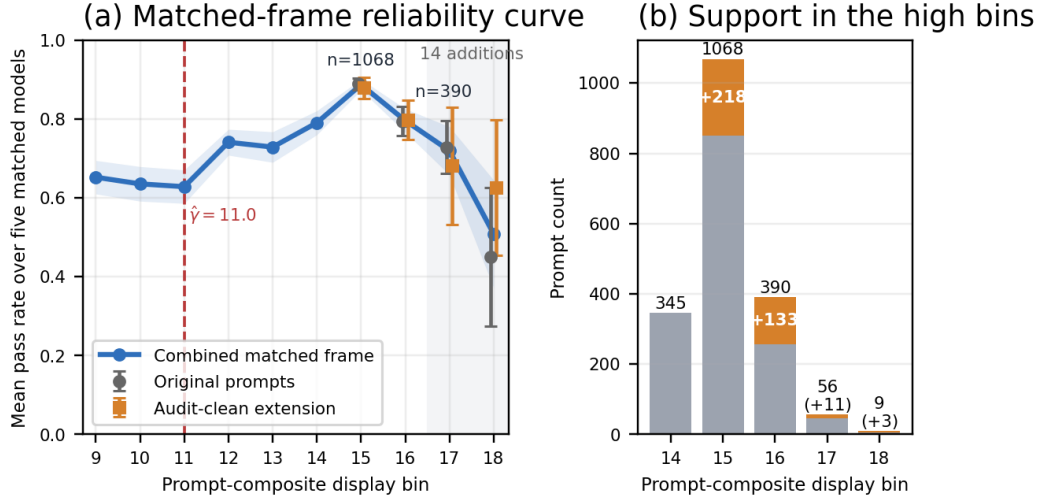
Figure 3: Audit-clean extension in a matched five-model frame, on raw harness outcomes. (a) Pass rate is first averaged over the five models shared by the original benchmark and extension, then over prompts within display bins, where bin b contains C_i \in [b - 0.5, b + 0.5) . Error bars and the shaded band are prompt-level normal-approximation intervals using \pm 1.96 standard errors. The dashed line is the matched-panel threshold estimated on the unbinned composite. (b) The 365 additions materially raise support at bins 15 and 16. Only 14 additions lie above 16, so bins 17 and 18 remain descriptive.
