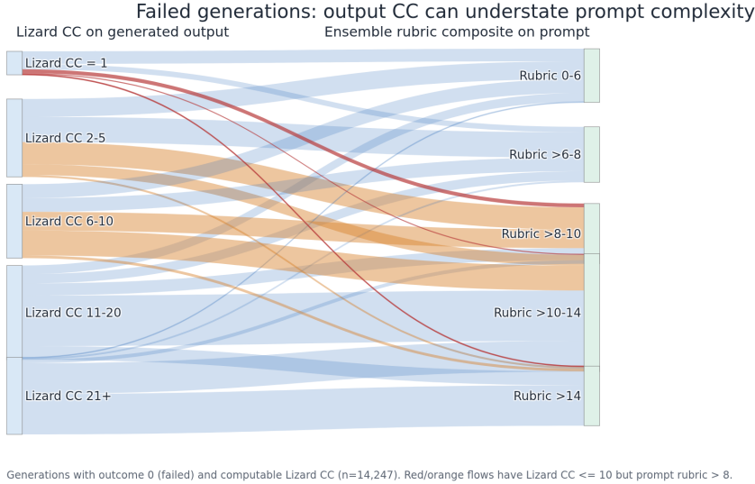
Figure 6: Reverse Threshold Problem among 14,247 failed generations (outcome 0) with computable Lizard CC. Generated-output complexity is on the left and the prompt composite is on the right. Highlighted flows have output CC \leq 10 and prompt composite > 8 .
