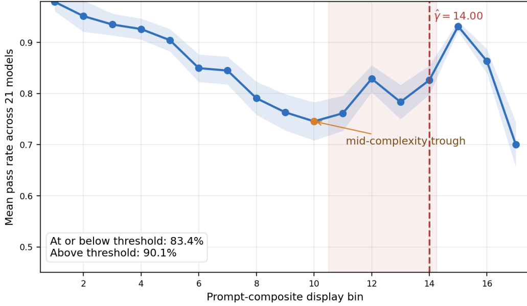
Figure 2: Unadjusted mean-pooled relationship in the original 5,000-prompt benchmark. Pass rate is first averaged across 21 models within prompt. Display bin b contains C_i \in [b - 0.5, b + 0.5) , so exact half-point boundaries enter the higher bin. The dashed line marks the threshold \hat{\gamma} = 14.0 estimated from the unbinned composite; the shaded vertical band is the 95% pairs-bootstrap interval. Bin 17 contains only 45 prompts and is descriptive; bins 0, 18, and 19 (3, 6, and 5 prompts) are omitted. This figure does not include task-type or construction-frame controls, or the separate 365-prompt extension.
