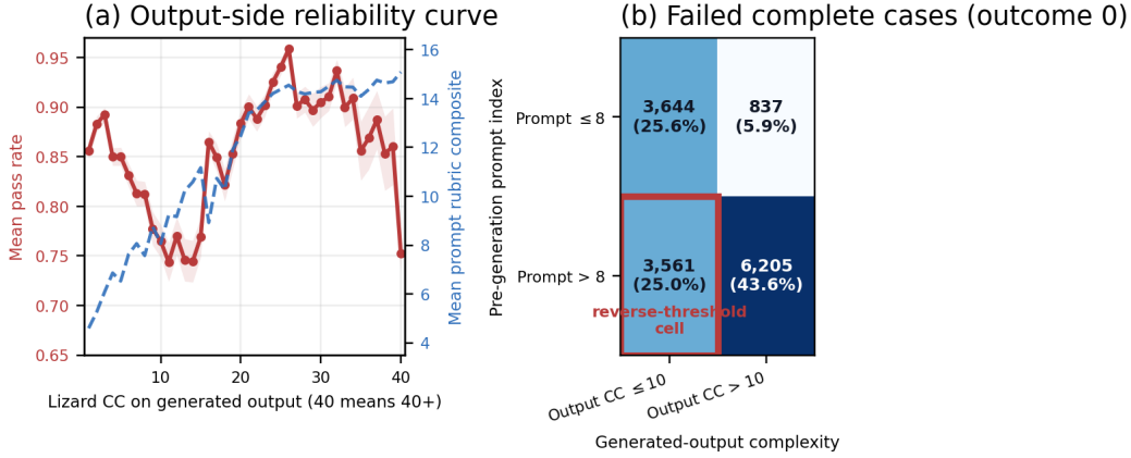
Figure 1: Generated-output complexity is failure-dependent. (a) Across 103,948 complete-case generations, points show mean pass rate by integer Lizard output CC; the shaded descriptive band is \pm 1.96 generation-row standard errors and does not adjust for repeated prompts or models. Here 40 denotes CC \geq 40 . The dashed blue line is the conditional mean prompt composite, read on the right axis. (b) Among failed complete cases (outcome 0), the outlined cell contains 3,561 of 14,247 generations (25.0%): the prompt composite is > 8 while generated-output CC is \leq 10 .
