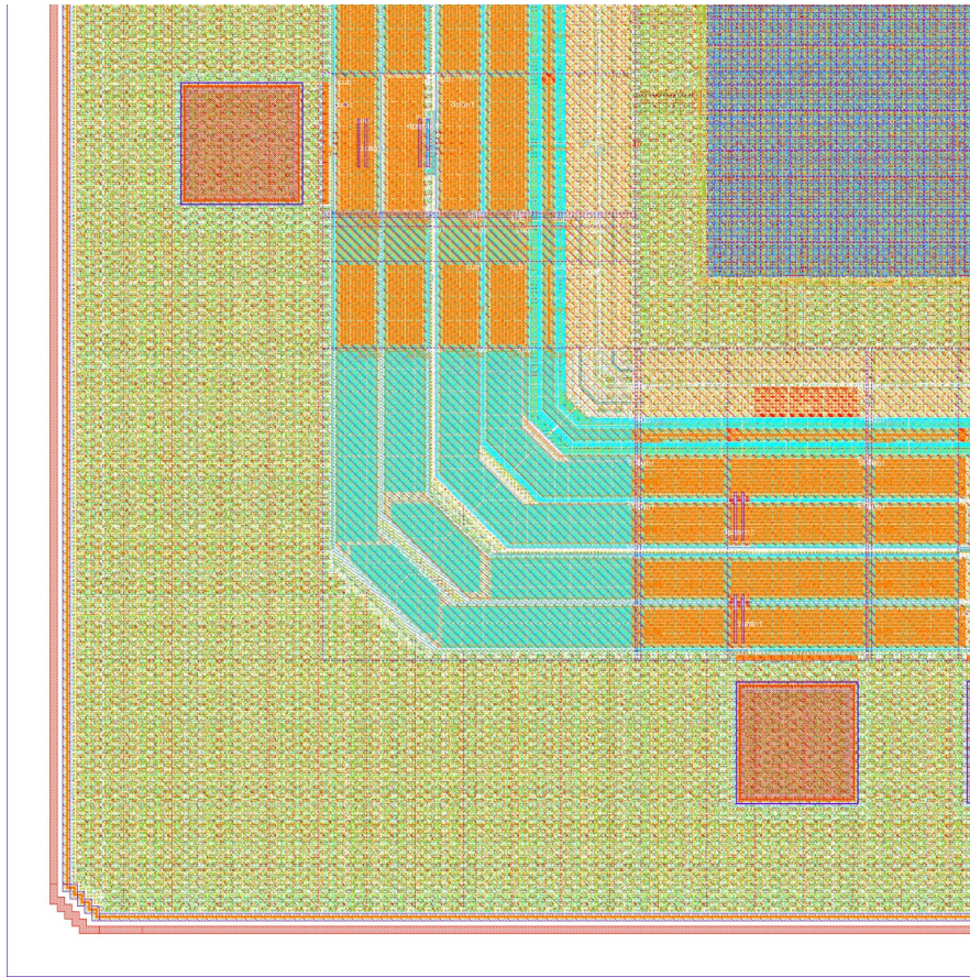
Figure 14. The lower left corner, 560 \mu\text{m} across. From the outside in: the seal ring, two bond pads, the pad ring's corner cell and the core edge. The fine pattern is metal fill.
