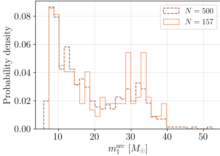
Figure 4.3: Distribution of the primary source-frame mass m_1^{\text{src}} for the full detectable population ( N = 500 , dashed) and the final injection set ( N = 157 , solid). The shape reflects the LIGO O3 Power Law + Gaussian population model adopted by LER v0.4.2. The duty cycle and SNR selection preferentially retains events with m_1^{\text{src}} in the 25–35 M_\odot range, consistent with higher-mass systems producing intrinsically louder signals and thus being more robust to the loss of detector uptime, while the high-mass tail above \sim 40 M_\odot is largely absent from the filtered population.
