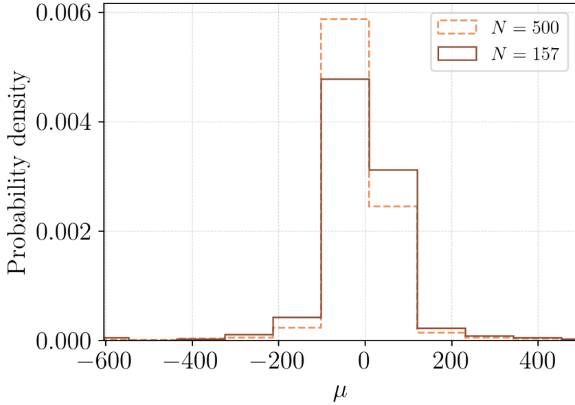
Figure 4.6: Distribution of image magnifications \mu for the full detectable population ( N = 500 , dashed) and the final injection set ( N = 157 , solid), prior to the duty cycle filter for the former and after it for the latter. Negative values correspond to Type II images (saddle points of the Fermat potential), which have mirror-inverted parity and acquire a \pi/2 Morse phase shift (see §3.3). The distribution is strongly peaked near \mu \sim 0 with extended tails; the horizontal axis is clipped to the 0.5–99.5 percentile range of the combined data to make the shape of the peak and tails visible, excluding a small number of extreme outliers reaching |\mu| \sim 10^3 .
