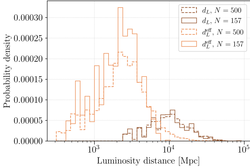
Figure 4.5: Comparison of the true luminosity distance d_L and the effective luminosity distance d_L^{\text{eff}} , for the full detectable population ( N = 500 , dashed lines) and the final injection set ( N = 157 , solid lines). Brown lines show d_L and orange lines show d_L^{\text{eff}} . Because magnification boosts the observed signal amplitude, d_L^{\text{eff}} = d_L/\sqrt{|\mu|} is systematically smaller than the true distance, shifting the effective-distance distributions toward lower values relative to d_L .
