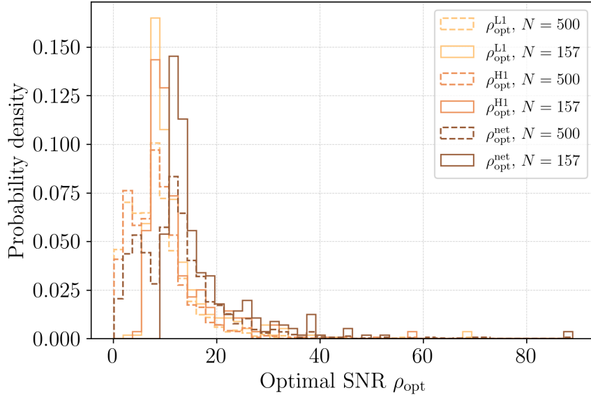
Figure 4.2: Distribution of optimal SNR for L1 ( \rho_{\text{opt}}^{\text{L1}} , light orange), H1 ( \rho_{\text{opt}}^{\text{H1}} , orange), and the network ( \rho_{\text{opt}}^{\text{net}} , brown), for the full detectable population ( N = 500 , dashed) and the final injection set ( N = 157 , solid) after the duty cycle and SNR filters. The network SNR distribution for the filtered population is truncated at \rho_{\text{net}} = 10 by construction, and its peak shifts to higher SNR relative to the full population, reflecting the removal of images that fall below the threshold once only the active detectors are considered. The individual L1 and H1 distributions can extend below \rho = 10 even after filtering, since the selection criterion applies to the network SNR rather than to each detector separately.
