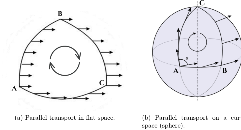
Figure 1.5: Comparison between parallel transport in flat and curved spaces. In flat space, the vector returns unchanged after a closed loop; in curved space, the final result depends on the path taken, revealing the manifold’s intrinsic geometry. Original illustrations based on the sources: [33, 40].
