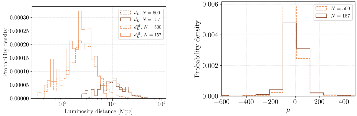
Figure 4.3: Left: true luminosity distance d_L (brown) versus effective luminosity distance d_L^{\text{eff}} (orange). Right: image magnification \mu .
