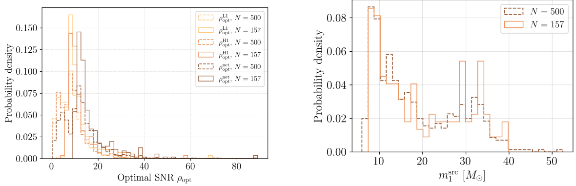
Figure 4.2: Left: optimal SNR for L1 ( \rho_{\text{opt}}^{\text{L1}} , light orange), H1 ( \rho_{\text{opt}}^{\text{H1}} , orange), and the network ( \rho_{\text{opt}}^{\text{net}} , brown). Right: primary source-frame mass m_1^{\text{src}} .
