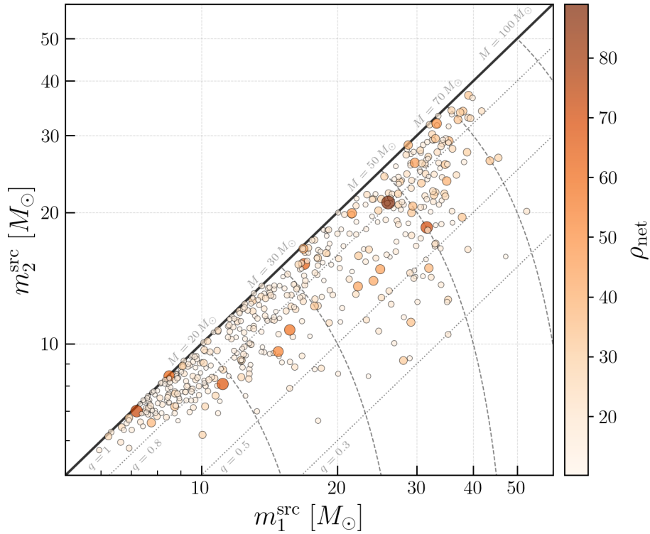
Figure 4.4: Source-frame component masses m_1^{\text{src}} and m_2^{\text{src}} for the 500 detectable lensed BBH events selected by LER, colour-coded by network SNR \rho_{\text{net}} . Diagonal dashed lines mark constant total mass M and dotted lines mark constant mass ratio q . The population traces the underlying LIGO O3 Power Law + Gaussian model (§4.1), with most events clustering near q = 1 and the highest-SNR events concentrated around M \sim 50\text{--}70 M_\odot .
