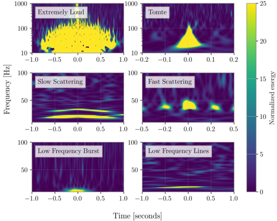
Figure 2.11: Time-frequency spectrograms of representative glitch classes recorded at LHO and LLO. Slow and Fast Scattering artefacts are attributed to light scattered by optics under increased ground motion, while the origin of Extremely Loud, Tomte, Low Frequency Burst, and Low Frequency Lines glitches remains unidentified. Source: [100].
