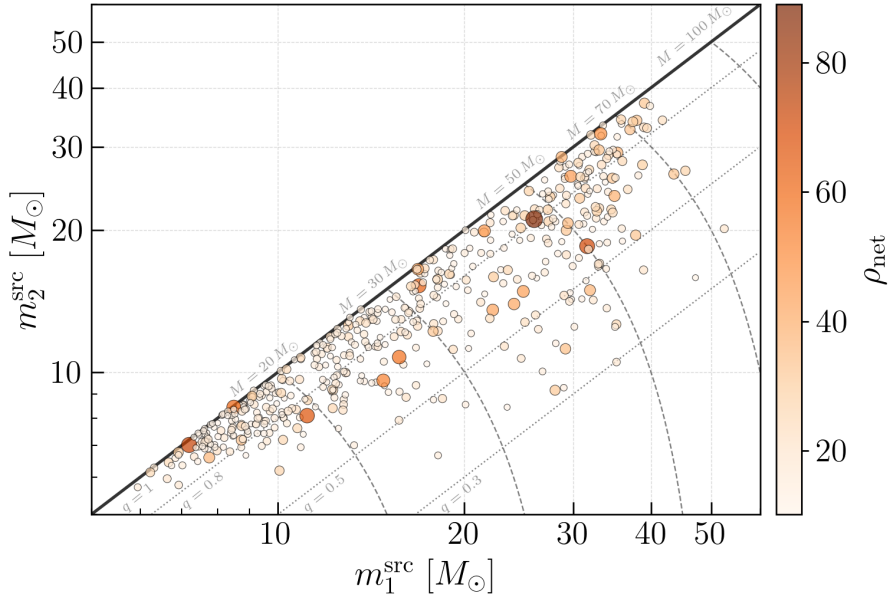
Figure 4.5: Source-frame component masses m_1^{\text{src}} and m_2^{\text{src}} for the 500 detectable lensed BBH events selected by LER, colour-coded by network SNR \rho_{\text{net}} . Dashed lines mark constant total mass M and dotted lines mark constant mass ratio q . The population traces the underlying LIGO O3 Power Law + Gaussian model (§4.1), with most events clustering near q = 1 and the highest-SNR events concentrated around M \sim 50\text{-}70 M_\odot .
