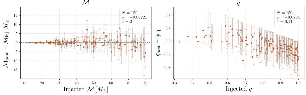
Figure 5.3: Left : chirp mass residual \mathcal{M}_{\text{post}} - \mathcal{M}_{\text{inj}} . Right : mass ratio residual q_{\text{post}} - q_{\text{inj}} . Both as a function of the injected value, for all 150 events.
