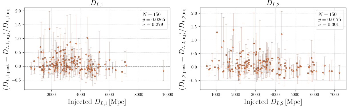
Figure 5.6: Left : relative residual for image 1, (D_{L,1,\text{post}} - D_{L,1,\text{inj}})/D_{L,1,\text{inj}} . Right : same for image 2. Both as a function of the injected value, for all 150 events.
