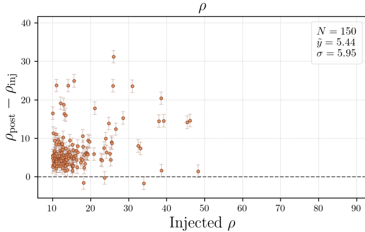
Figure 5.7: Difference between the posterior-recovered network SNR \rho_{\text{post}} (median of the combined network SNR recomputed from the joint posterior samples, §5.4) and the injected network SNR \rho_{\text{inj}} (computed by LER, §4.1), as a function of \rho_{\text{inj}} , for the N = 150 successfully analyzed events. The offset is systematically positive (median 5.44, \sigma = 5.95 ).
