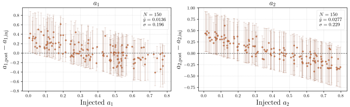
Figure 5.5: Left : primary spin residual a_{1,\text{post}} - a_{1,\text{inj}} . Right : secondary spin residual a_{2,\text{post}} - a_{2,\text{inj}} . Both as a function of the injected value, for all 150 events.
