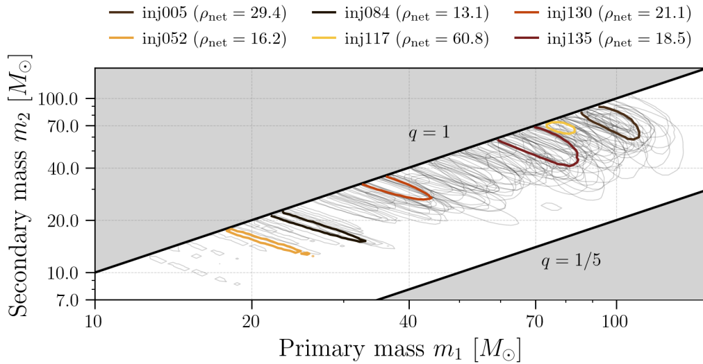
Figure 5.2: Recovered 90% credible (m_1, m_2) contours for six events spanning the sample’s network SNR range (colored), against the 90% credible contours of all other events (grey). The shaded regions mark q < 1/5 and q > 1 , outside the astrophysical mass ratio range considered here.
