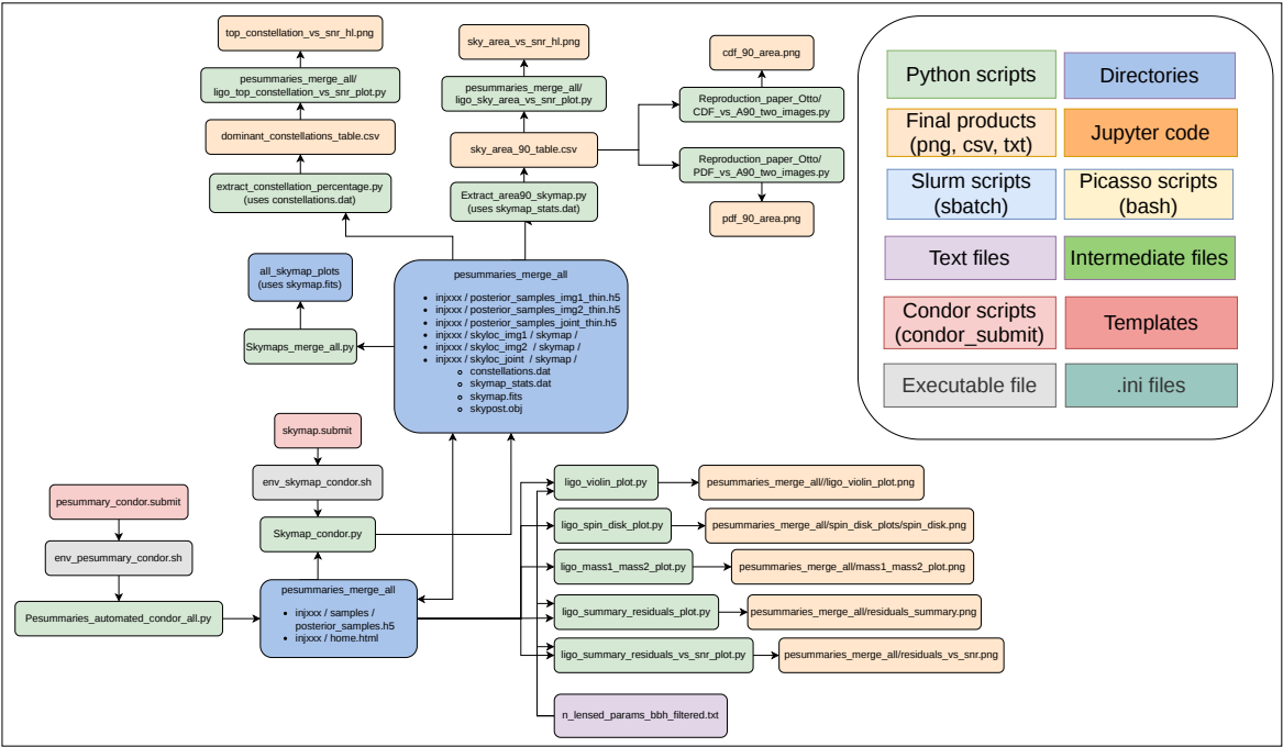
Figure C.2: Detailed implementation of the CIT (HTCondor) post-processing branch of the pipeline, referenced in §5.4 and §6.1. An interactive version with clickable links to each script is available at https://github.com/XxavierGarcia/TFM_reproducibility_material/blob/main/diagrama_pipeline.drawio.pdf (download to enable links).
