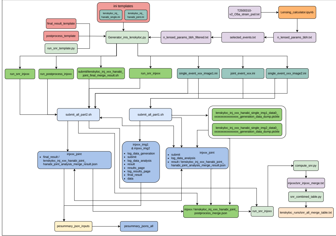
Figure C.1: Detailed implementation of the Picasso (SLURM) branch of the pipeline, referenced in §5.4. An interactive version with clickable links to each script is available at https://github.com/XxavierGarcia/TFM_reproducibility_material/blob/main/diagrama_pipeline.drawio.pdf (download to enable links).
