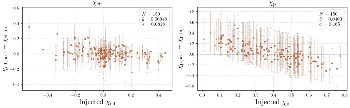
Figure 5.4: Left : effective spin residual \chi_{\text{eff,post}} - \chi_{\text{eff,inj}} . Right : precessing spin residual \chi_{\text{p,post}} - \chi_{\text{p,inj}} . Both as a function of the injected value, for all 150 events.
