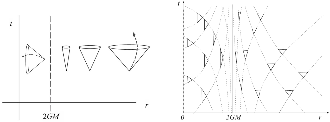
(a) Tilting of light cones in Schwarzschild coordinates. The arrows illustrate possible world-lines of particles.
