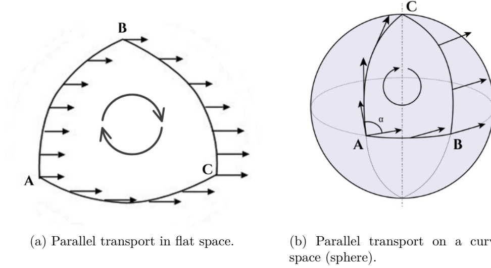
Figure 1.7: Comparison between parallel transport in flat and curved spaces. In flat space, the vector returns unchanged after a closed loop; in curved space, the final result depends on the path taken, revealing the manifold's intrinsic geometry. Original illustrations based on the sources: [Llibre_Peter_Collier_unacosadificildecomprender, ParallelTransportSvg].
