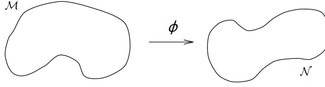
Figure 1.4: Illustration of a mapping \phi : \mathcal{M} \rightarrow \mathcal{N} between two sets, where each element of \mathcal{M} is assigned precisely one element of \mathcal{N} . Source: [llibrecarroll2004lectures].
