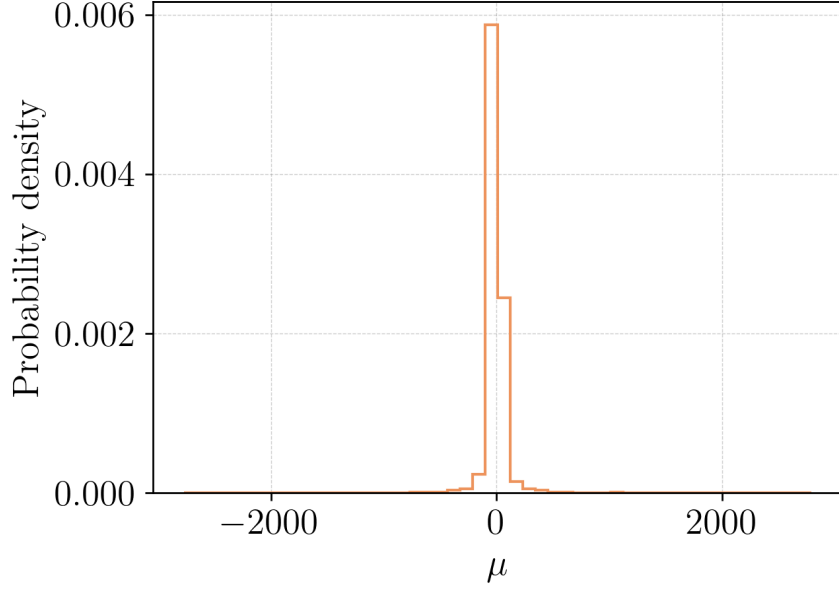
Figure 4.4: Distribution of image magnifications \mu for the lensed population prior to the duty cycle filter. Negative values correspond to Type II images (saddle points of the Fermat potential), which have mirror-inverted parity and acquire a \pi/2 Morse phase shift (see §3.3). The distribution is strongly peaked near |\mu| \sim 1 with extended tails at large |\mu| , consistent with the SIS power-law magnification prior adopted by LER.
