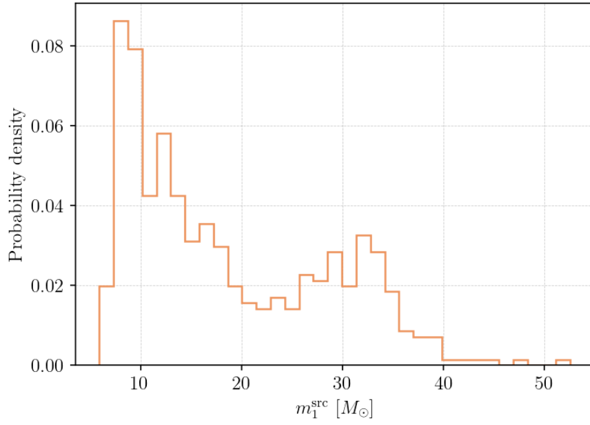
Figure 4.2: Distribution of the primary source-frame mass m_1 for the 157 injected lensed BBH events. The shape reflects the LIGO O3 Power Law + Gaussian population model adopted by LER v0.4.2, with a dominant low-mass component and a secondary feature near 30 M_\odot from the Gaussian component.
