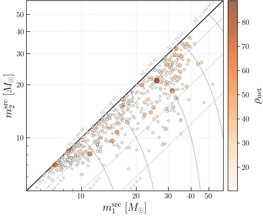
Figure 4.3: Source-frame component masses m_1^{\text{src}} and m_2^{\text{src}} for the 500 detectable lensed BBH events selected by LER, colour-coded by network SNR \rho_{\text{net}} . Diagonal dashed lines mark constant total mass M and dotted lines mark constant mass ratio q . The population traces the underlying LIGO O3 Power Law + Gaussian model (§4.1), with most events clustering near q = 1 and the highest-SNR events concentrated around M \sim 50\text{--}70 M_\odot .
