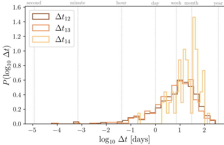
Figure 4.5: Distribution of time delays \Delta t between the two lensed images for the 157 injected events, shown on a logarithmic scale. The distribution spans from minutes to months, consistent with galaxy-scale lenses in the geometric optics regime. The Earth’s rotation during this interval is the primary mechanism enabling improved sky localization through joint analysis (§3.4.2).
