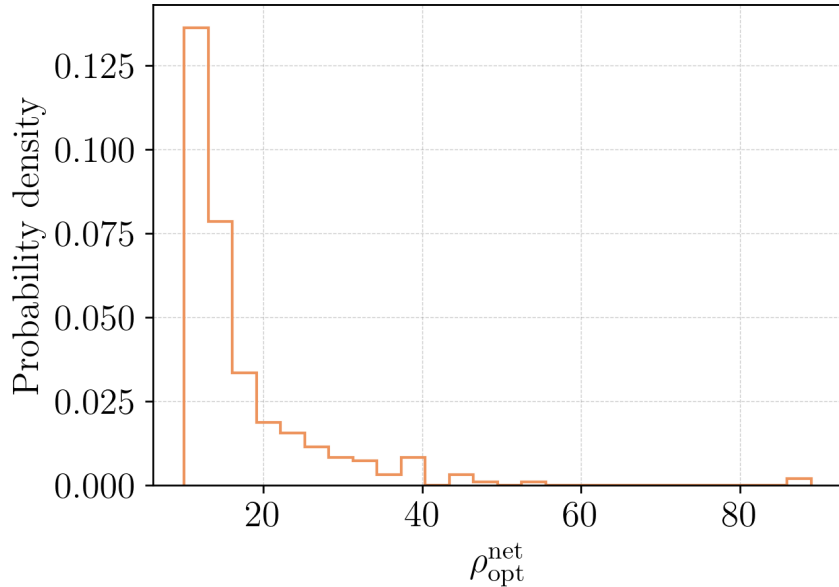
Figure 4.1: Distribution of network SNR \rho_{\text{net}} for the 157 injected lensed BBH events after the duty cycle filter. The distribution is truncated at \rho_{\text{net}} = 10 by construction and peaks just above the threshold, with a tail extending to higher values for strongly magnified or favorably oriented systems.
