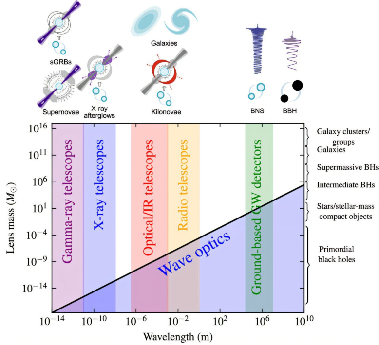
Figure 3.1: Illustration of the mass scales at which wave optics effects become relevant for gravitationally lensed signals. The geometric optics regime is valid when the wavelength of the radiation is much smaller than the scale of the lensing potential. The wave optics regime is valid when the wavelength is comparable to the scale of the lensing potential. Because the wavelength of GWs detected by the current ground-based detectors is typically much larger than the wavelength of most light sources, wave optics effects can become relevant for lenses below \leq 100M . Since other GW detectors like LISA will be sensitive to even longer wavelengths, wave optics effects will be even more important. The precise mass scale also depends on the lensing configuration, such as the distance from the caustic, where wave optics effects can become more prominent close to a caustic when the magnification is large. Credit: Philosophical Transactions of the Royal Society A: Mathematical, Physical and Engineering Sciences (2025). DOI: 10.1098/rsta.2024.0134.
