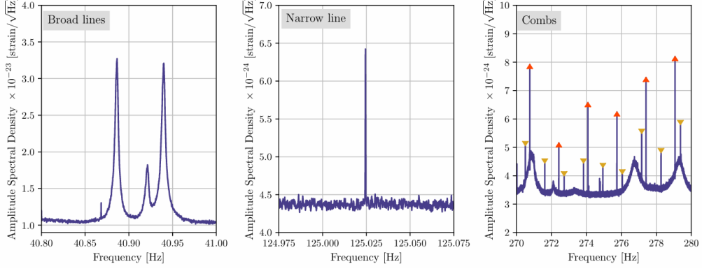
Figure 2.10: High-resolution amplitude spectral density ( \Delta f = 1/1800 Hz) of LIGO Hanford strain data illustrating three representative line artefacts. Left: a broad spectral feature associated with mirror suspension roll-mode resonances. Centre: an isolated narrow line of unknown origin. Right: two frequency combs with distinct spacings, marked by upright and inverted triangles, alongside broader noise structures. Source: [100].
