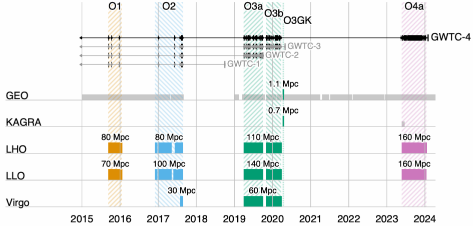
Figure 2.14: Timeline of LVK observing runs from the first detection in 2015 through O4a. Colored bars indicate the periods during which each detector was operating, together with the typical BNS inspiral range achieved in each run. GEO astrowatch and KAGRA O4a periods (light gray) were not included in the main GW analyses. Virgo joined the network in the final month of O2 and operated throughout O3; a short joint O3GK run also included GEO600 and KAGRA. Tick marks along the top indicate GW candidates from GWTC-1 through GWTC-4 with astrophysical probability \geq 50\% . Source: [112].
