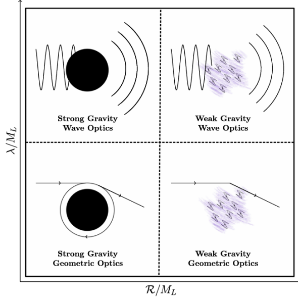
Figure 3.2: Diagram exemplifying the distinct regimes of GW lensing. We denote M_L the lens mass, R its characteristic size and, \lambda the wavelength of the incoming wave. In this work we are primarily concerned with the strong gravity, wave optics regime (top left), particularly in the application of BH perturbation theory to explore the phenomenology of GW distortions in this part of parameter space. We will also make an explicit connection to lensing characteristics in the weak gravity, wave optics regime (top right). Source: [148].
