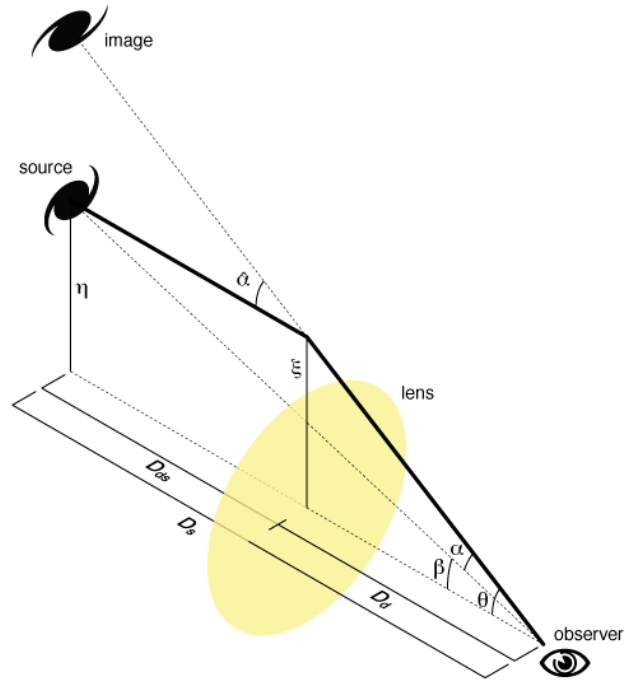
Figure 3.3: Geometry of gravitational lensing. Source: [159] .
