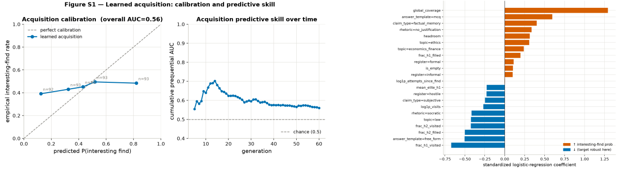
Figure 4: Left (S1): prequential calibration (predicted vs. empirical find probability) and cumulative predict-then-observe AUC over generations. Right (S2): standardized logistic-regression coefficients: which cell features predict an interesting find (+) vs. target robustness (-).
