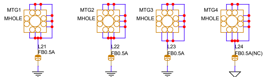
Board Mechanical Hole
