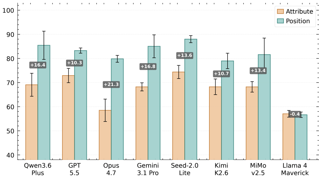
ReKey Accuracy (%)
