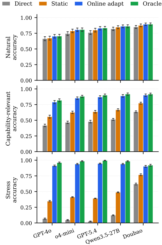
Figure 3: Online adaptation to distribution shift. Replay accuracy across five backbones and three stream constructions. Online adapt stays close to the Oracle upper bound and far above Static everywhere; the gap is largest under the stress protocol, where Direct nearly collapses. Error bars are seed std (50–200 seeds per cell).
