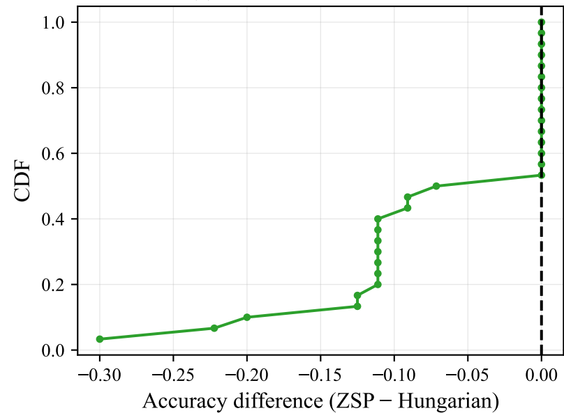
(c) Cumulative distribution
