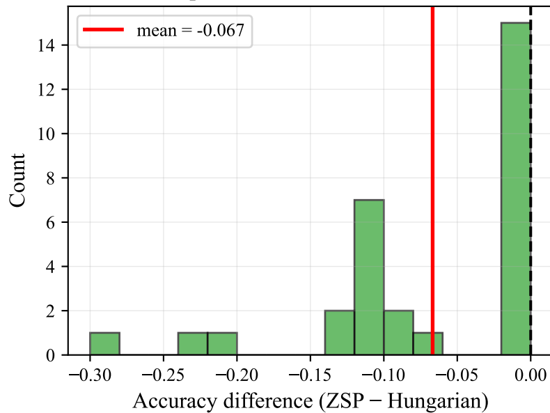
(b) Difference distribution p = 0.0001 , winner = 0%
