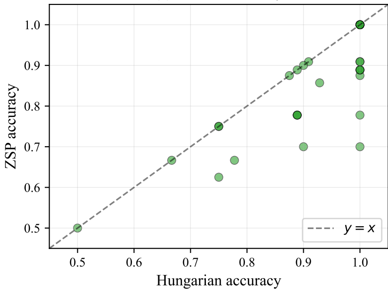
(a) Paired accuracy
