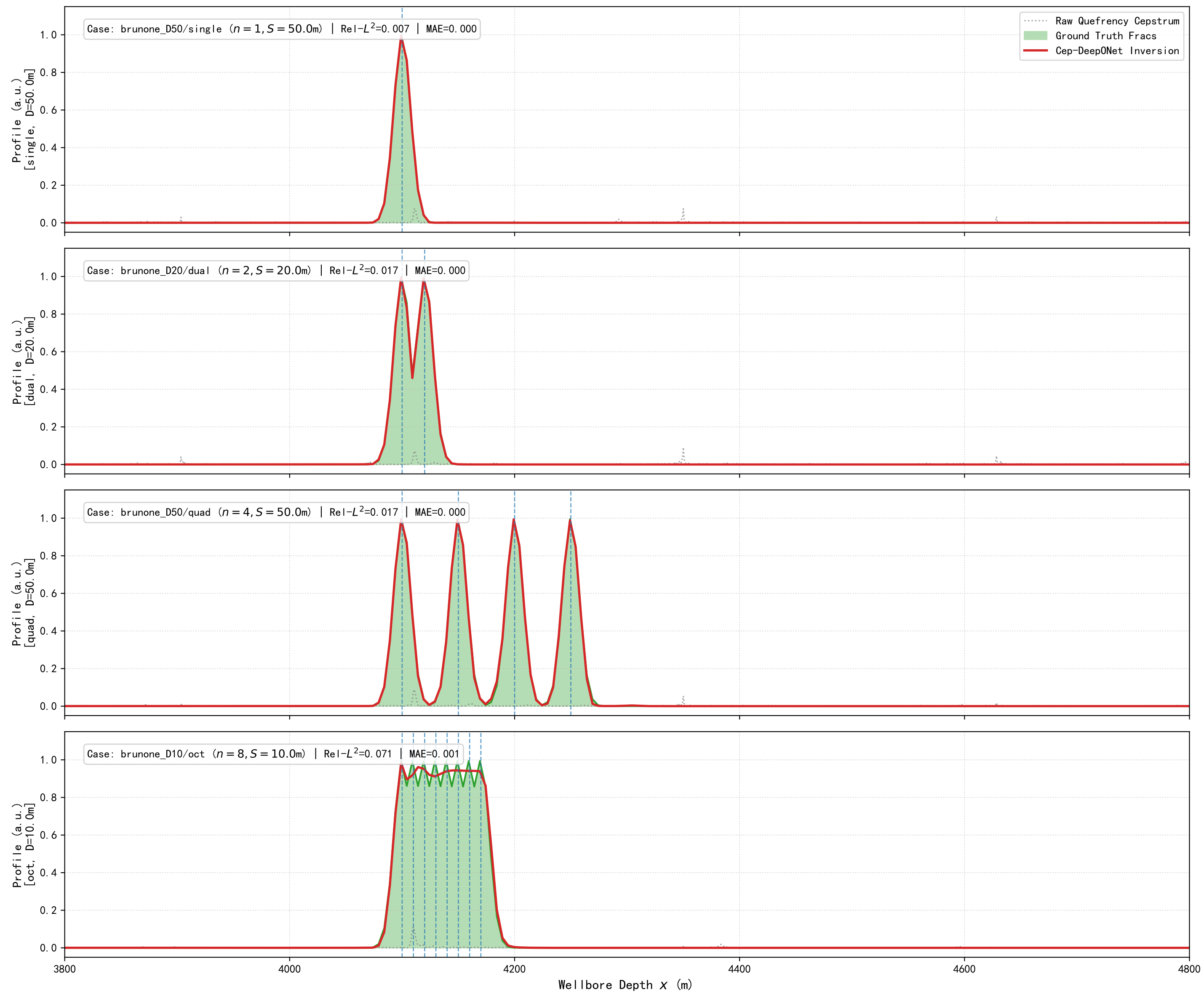
Cep-DeepONet Full Waveform Inversion vs Ground Truth &amp; Raw Cepstrum
