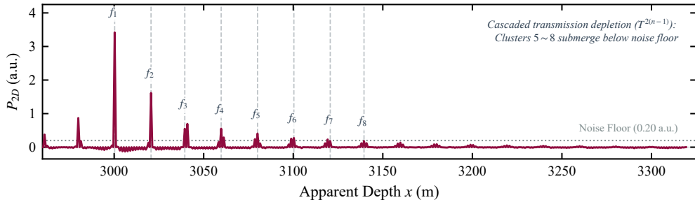
(d) Grade C: Deep Blind Zone / Multi-Interface Loss ( S = 20 m, n_{total} = 8 )
