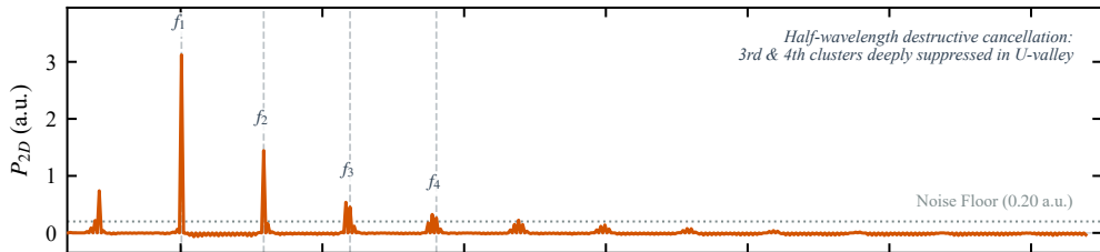
(d) Grade C: Deep Blind Zone / Multi-Interface Loss ( S = 20 m, n_{total} = 8 )
