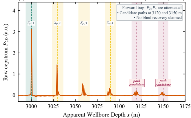
(c) Case 3: Deep Multi-Interface Depletion ( S = 20 m, n = 8 )
