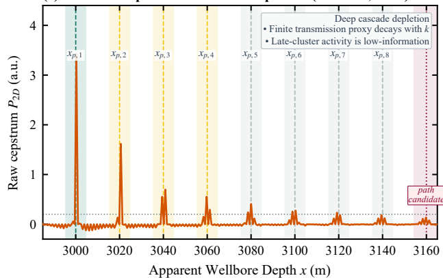
(c) Case 3: Deep Multi-Interface Depletion ( S = 20 m, n = 8 )
