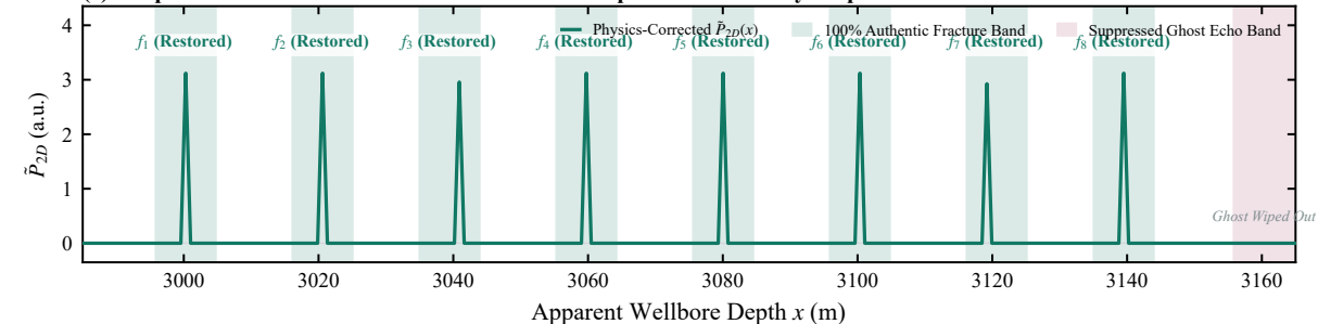
(e) Output: Reconstructed True Fracture Profile & Spatial Authenticity Map
