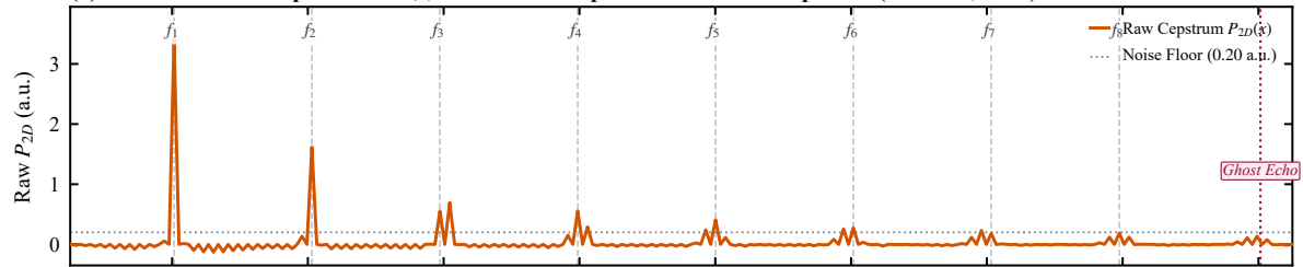
(b) Sub-Process 1: Multi-Path Reverberation & Harmonic Peeling Operator
