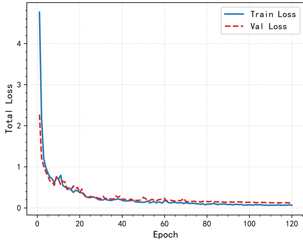
(a) Total Loss Convergence
