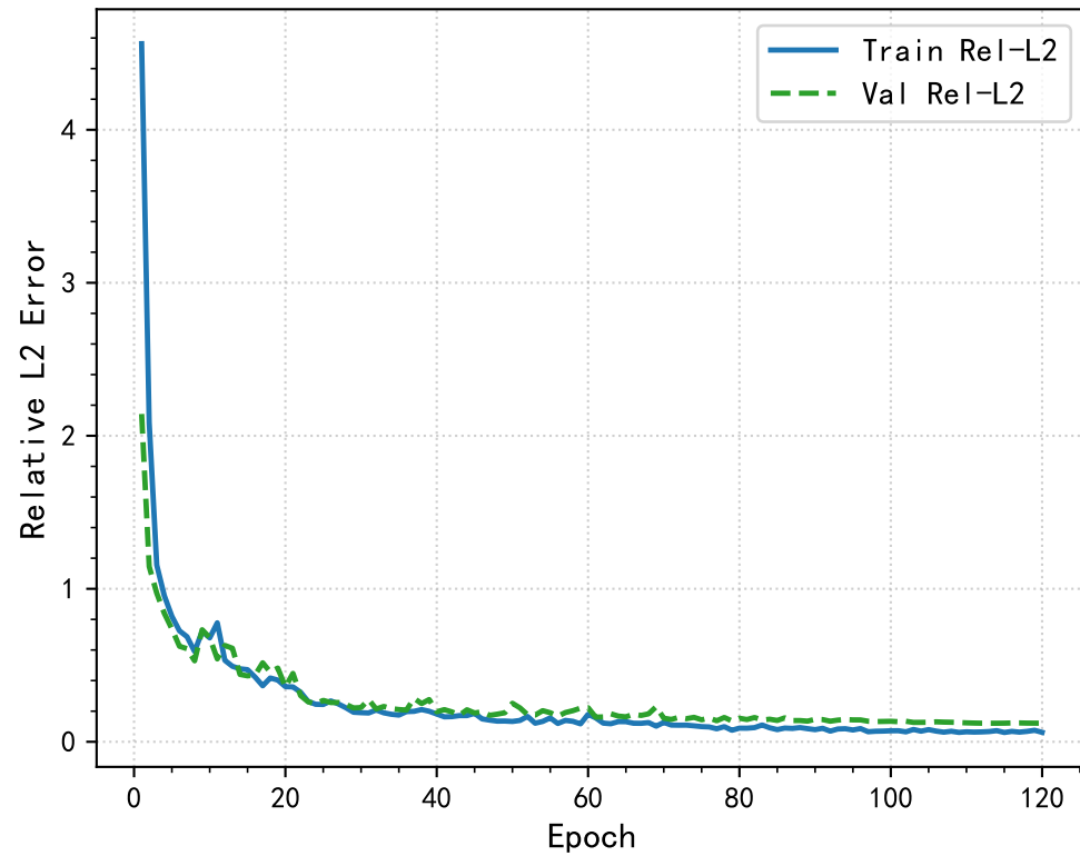
(b) Relative L^2 Norm Error
