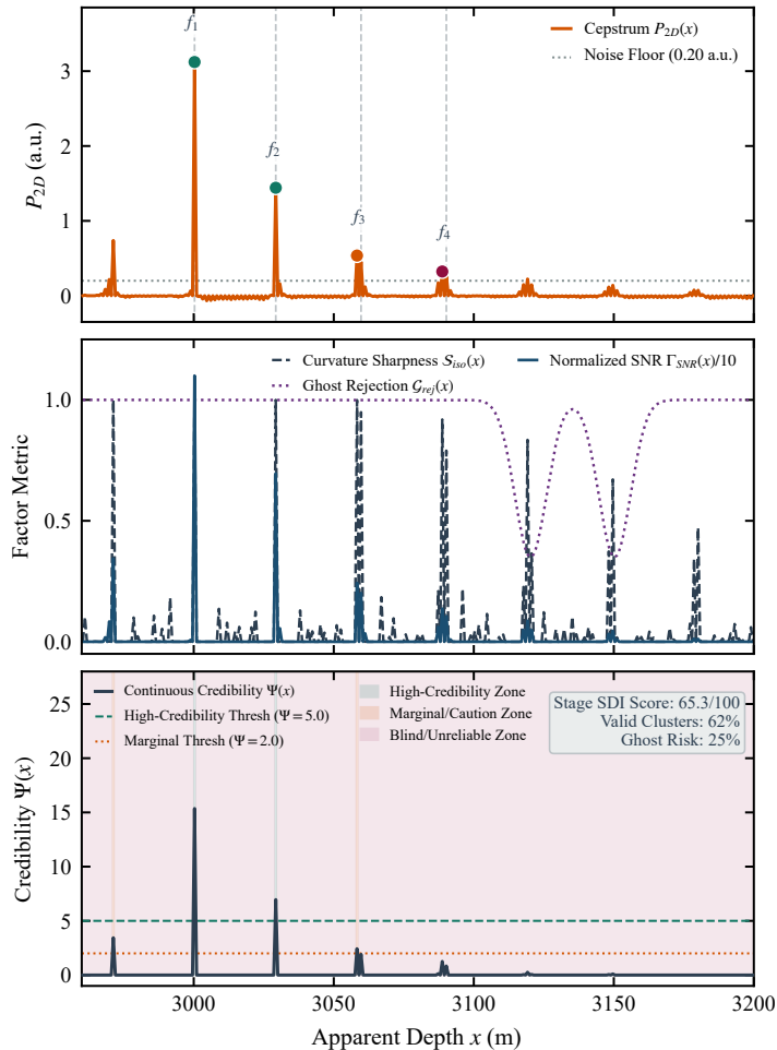
(b) Case 2: Phase Cancellation & Ghost Risk ( S = 30 m, n = 4 )
