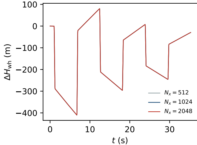
(b) three-grid p = 2.49
