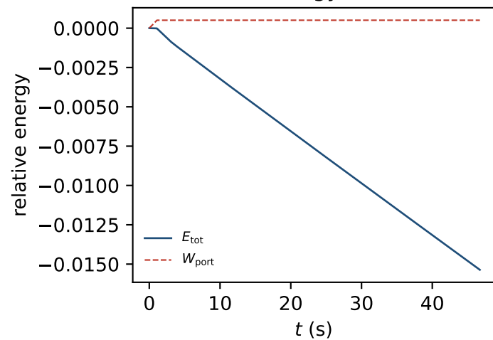
(c) energy audit
