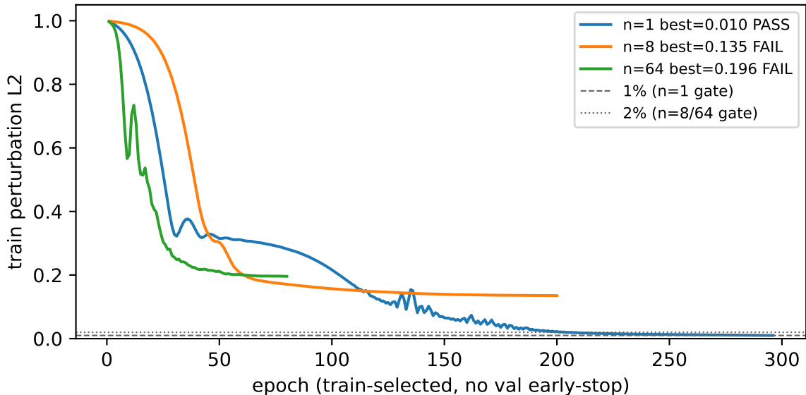
Round2 C1 overfit — QueryFourierMLP, seed=42
