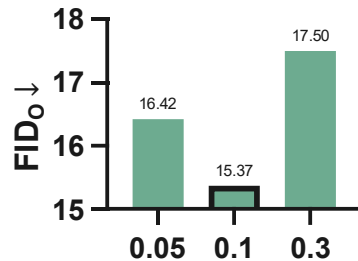
Base noise level \sigma
