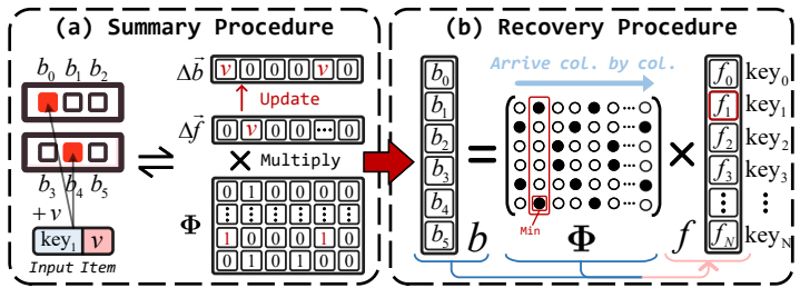
Figure 2: Matrix formulation of Count-Min. The linear sketching problem can be analyzed via simple matrix operations.
