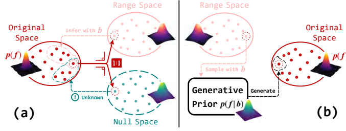
Figure 5: Illustration of our insights. (a) The GT f cannot be recovered due to orthogonal information loss in the null space. (b) We leverage GMs to generate the null-space component which is in harmony with the range-space component.
