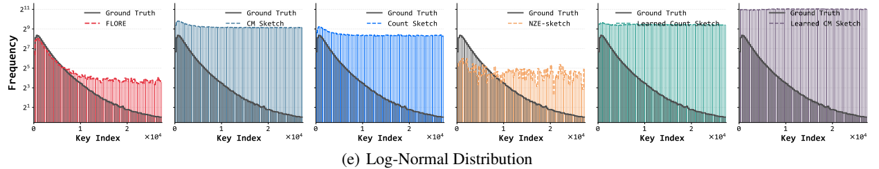
Figure 26: Visualizations of sketch recovery under a fixed 32KB memory budget. From left to right, we present the recovery results of FLORE, CM, CS, NZE, LCM, and LCS, compared against the ground-truth sample distribution. To enhance readability, every 100 consecutive keys are aggregated in the x-axis.
