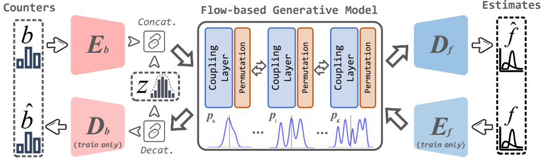
Figure 10: The architecture of FLORE. FLORE is modeled as an invertible mapping in the latent space.
