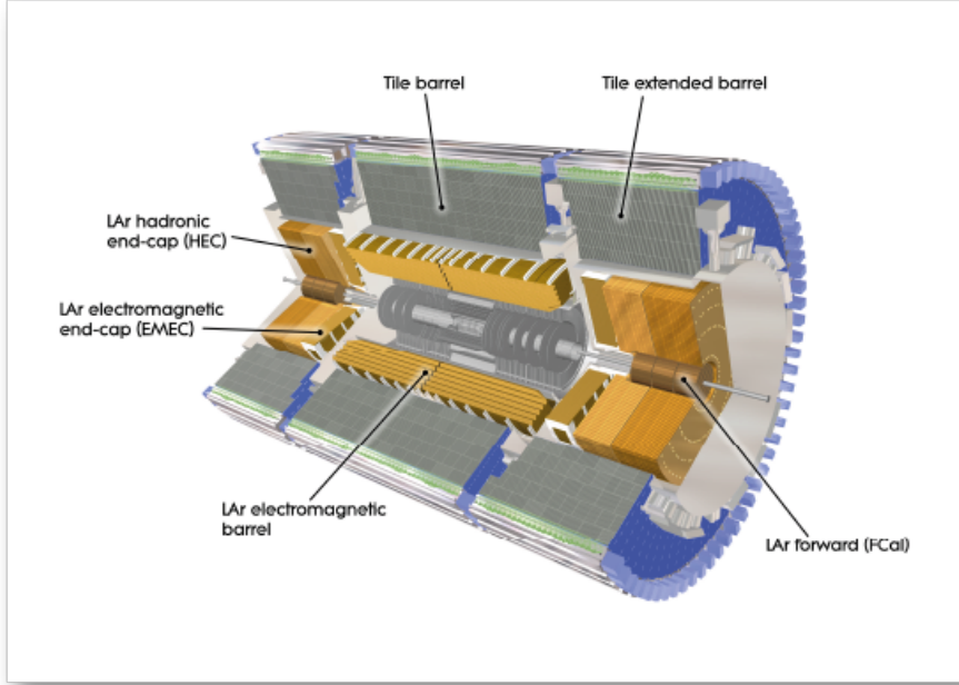
Figure 5. Schematic view of the Calorimeters ATLAS (2019b), showing the electromagnetic and hadronic calorimeters. Image credit: CERN .
