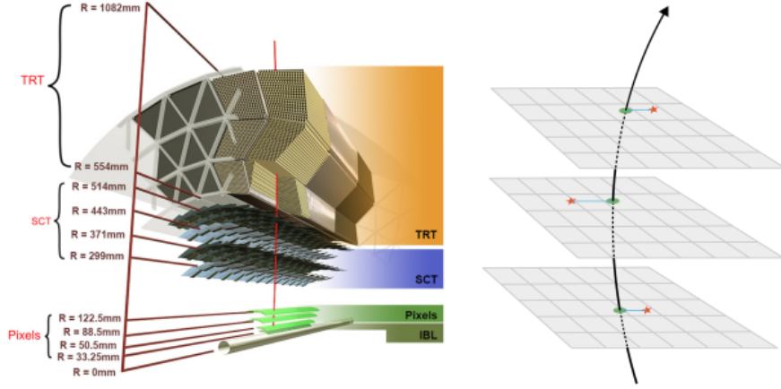
Figure 3. Schematic view of the Inner Detector ATLAS (2019b), showing the beam pipe, pixel barrel, SCT barrel, and TRT. Image credit: CERN .
