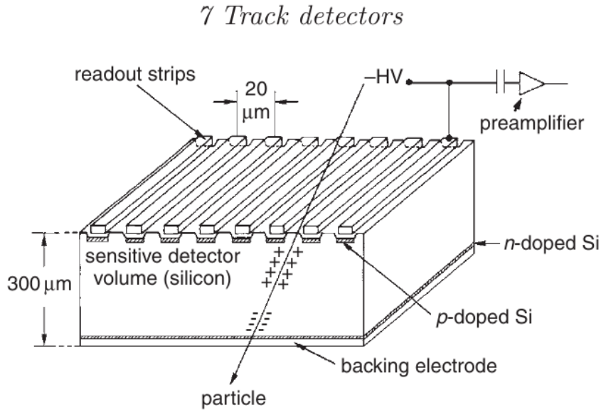
Figure 4. Schematic view of silicon microstrip detector. credit:
