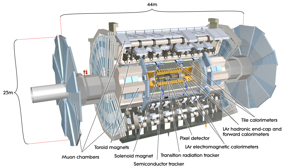
Figure 2. Schematic view of the ATLAS detectorATLAS (2019b), showing the main subsystems arranged around the interaction point. Image credit: CERN .
