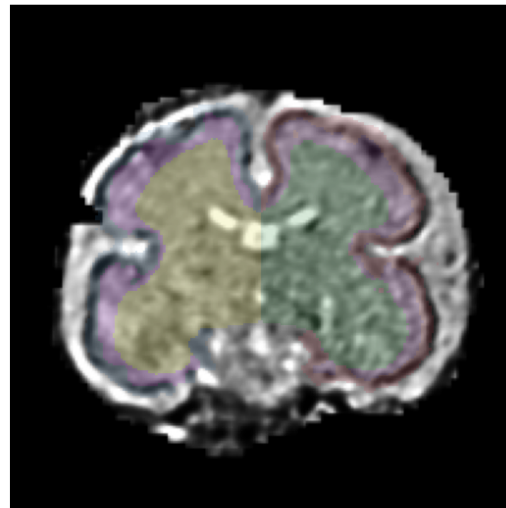
SP Model
