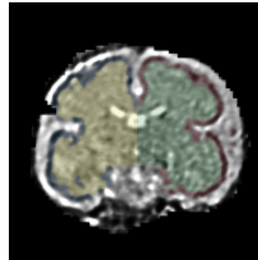
5-Label Model
