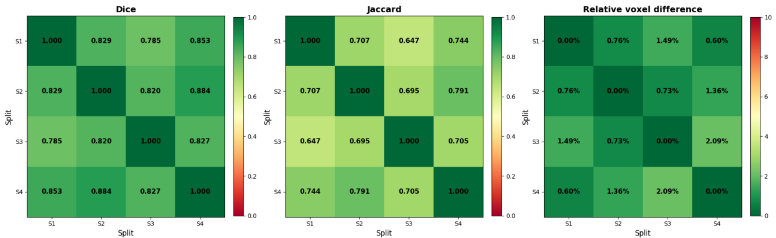
Cross-Split Reliability: Cortical Plate (5-Label Model) - FCB145
