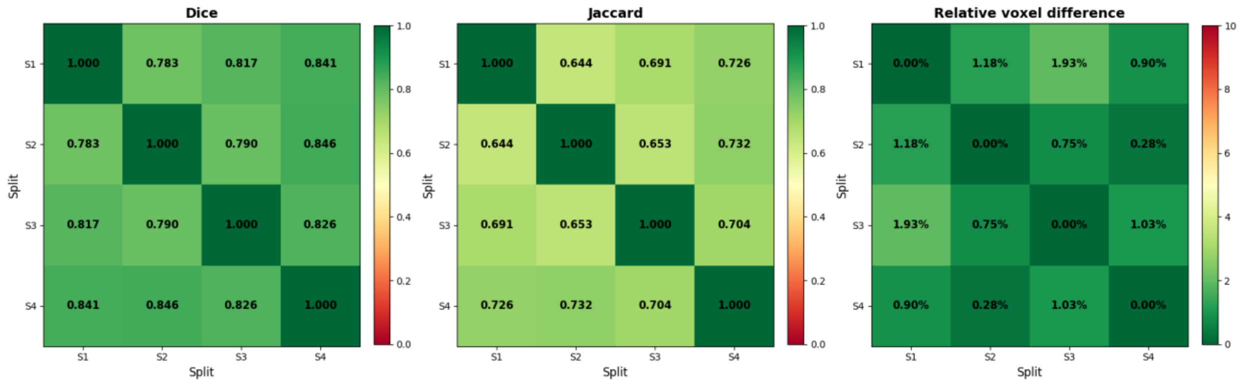
Cross-Split Reliability: Cortical Plate (SP Model) - FCB145
