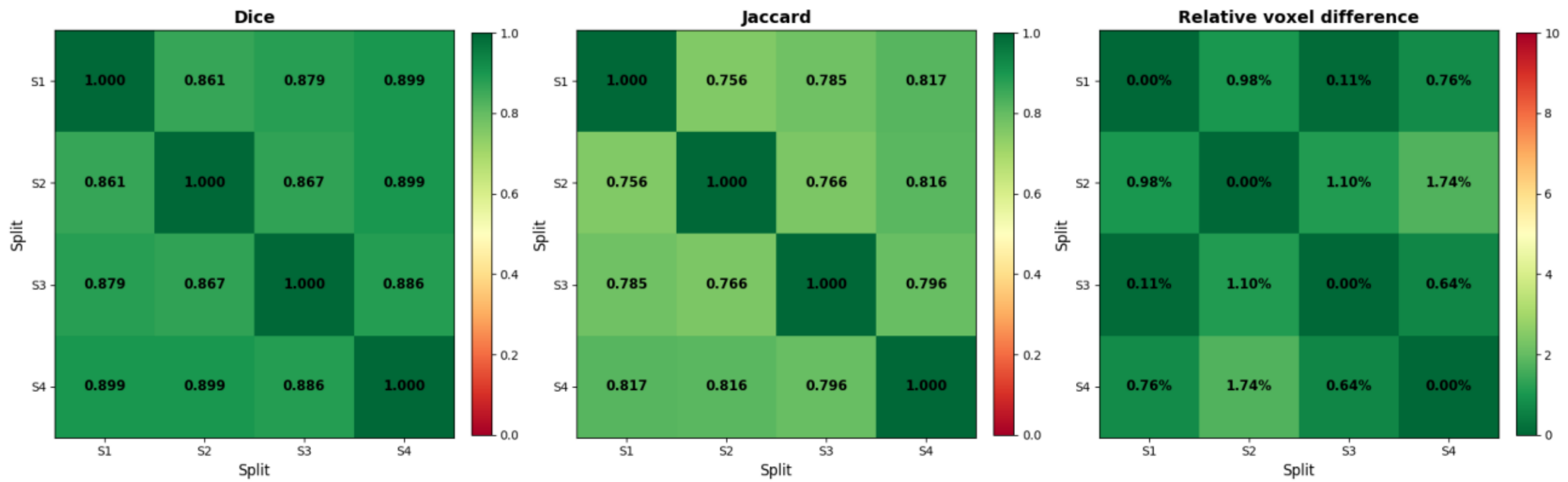
Cross-Split Reliability: Subplate (SP Model) - FCB145
