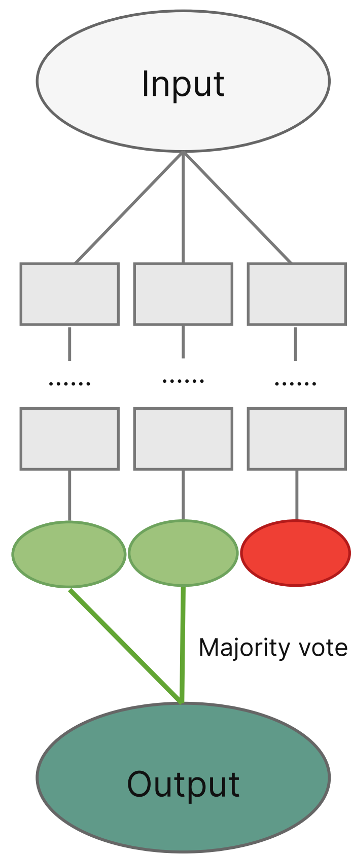
(c) Self Consistency with CoT ( CoT-SC )
