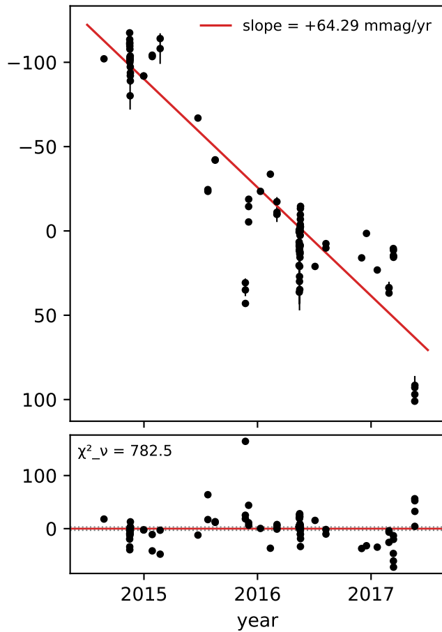
Strongest Trend Gaia DR3 382186599682713984 (G = 11.14, N = 97)
