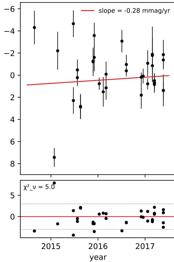
Brightest Star Gaia DR3 381669249398576896 (G = 8.26, N = 36)
