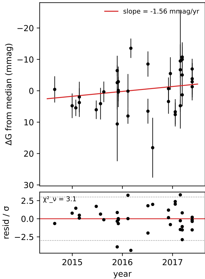
Average Star Gaia DR3 369118427247497728 (G = 16.67, N = 36)
