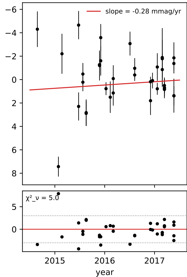
Brightest Star
