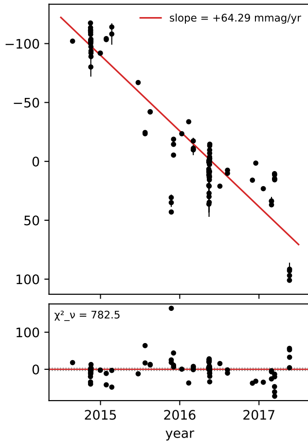
Strongest Trend
