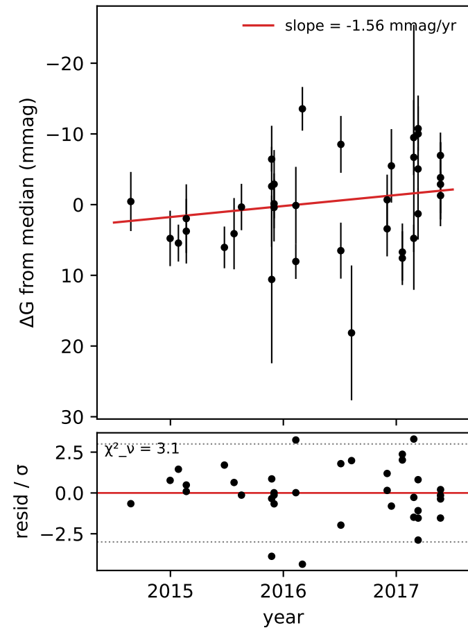
Average Star
