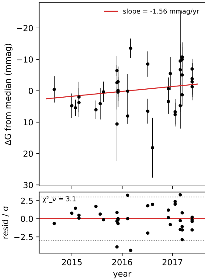
Average Star Gaia DR3 36911842724797728 (G = 16.67, N = 36)
