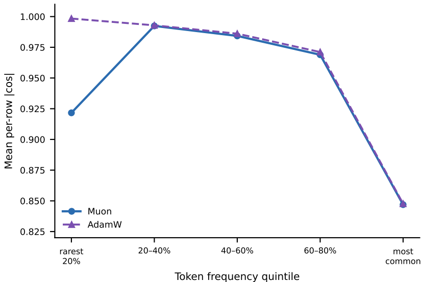
Rare tokens show higher per-row alignment (single run)
