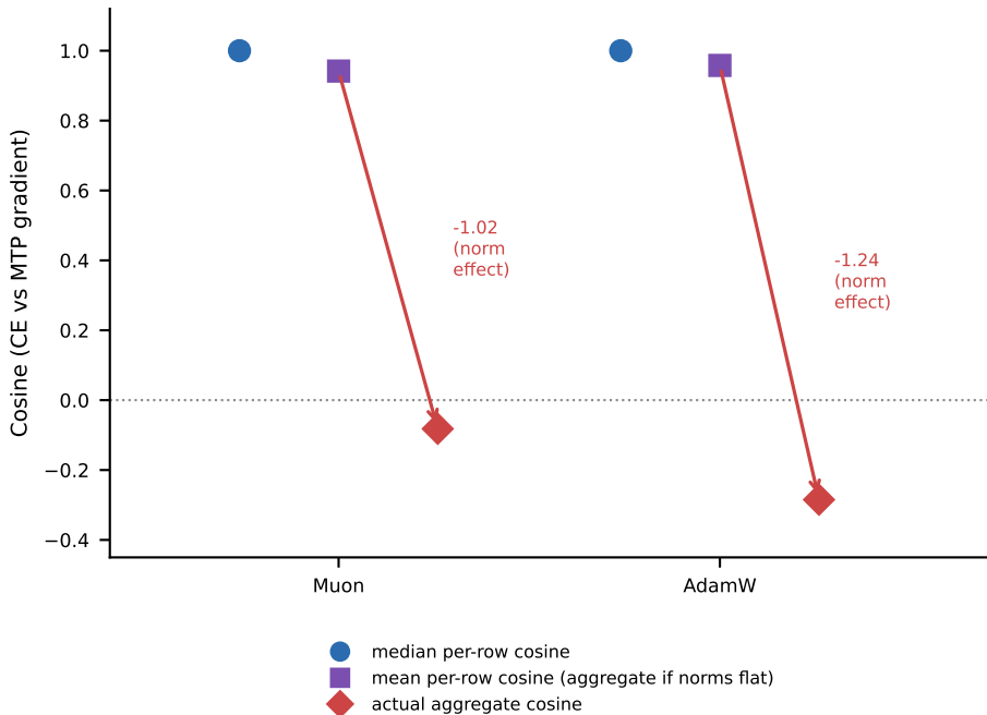
Per-row norm structure, not the typical cosine, sets the aggregate
