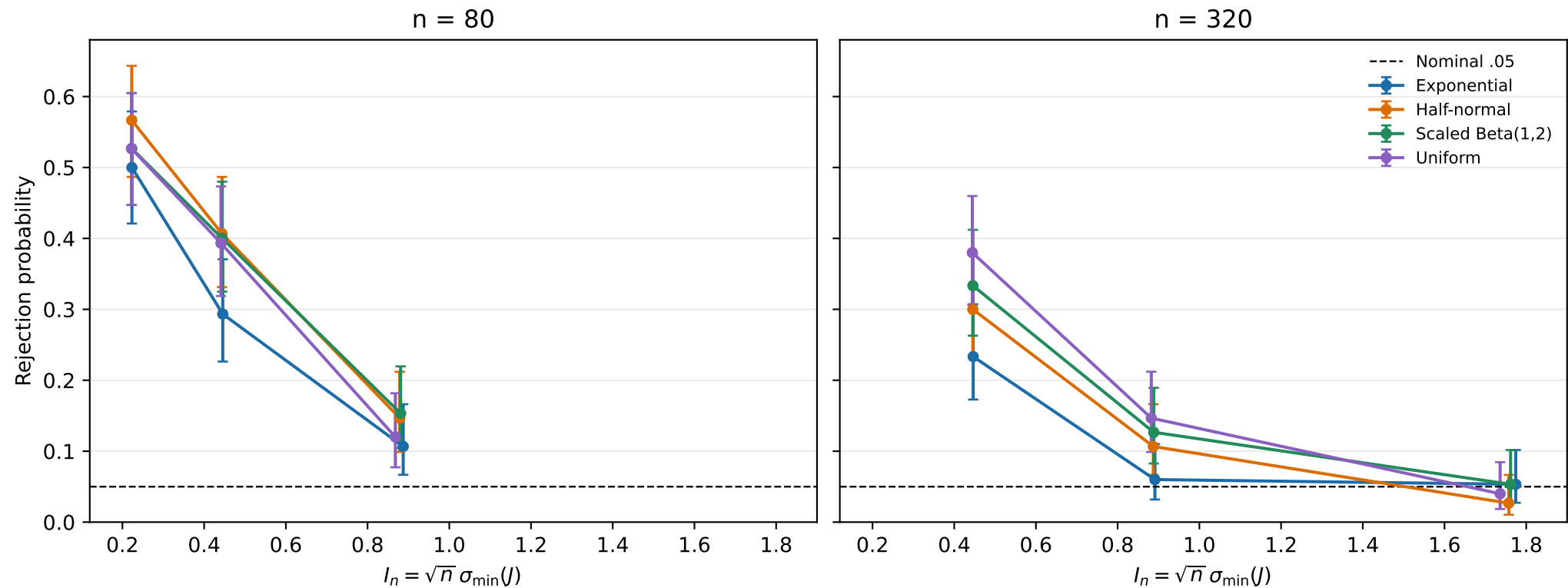
Figure 2. Frozen bridge transition: fully recomputed studentized-permutation evidence only (150 replications and 99 permutations per cell; empirical, not Wald-theorem validation)
