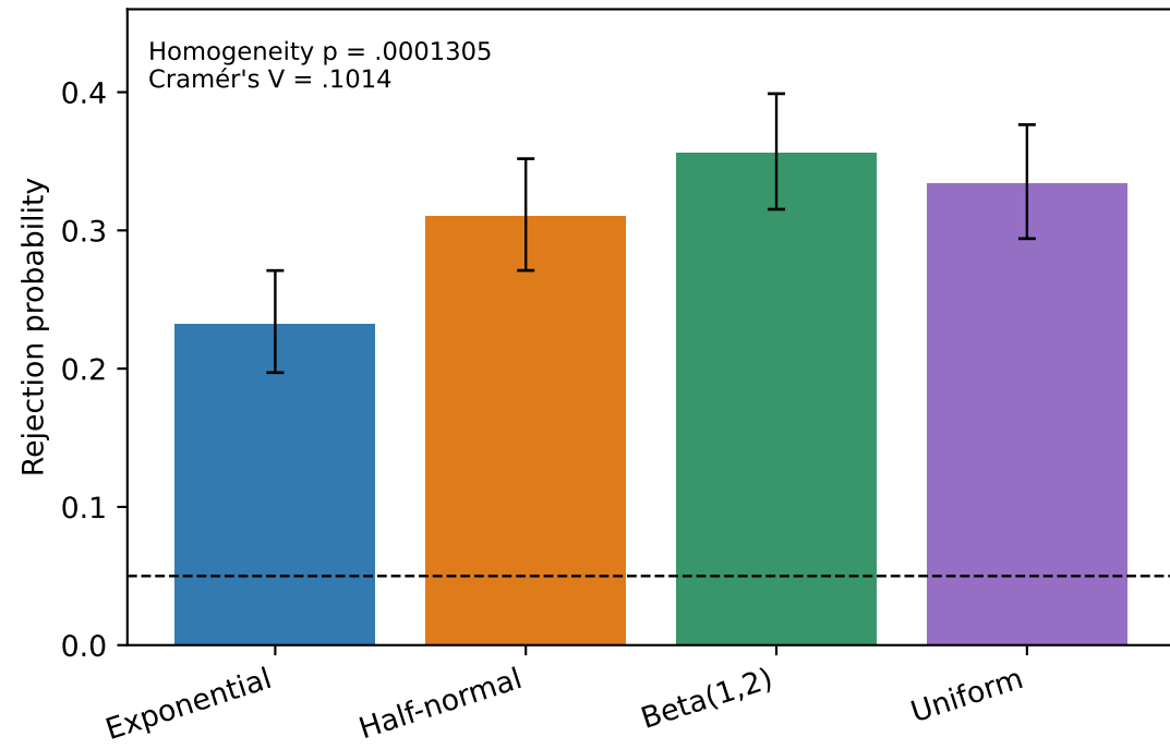
Figure 3. Family residuals unexplained by the index: studentized-permutation evidence only A. Legacy families at matched first-order index ( I_n \approx 0.445 )
