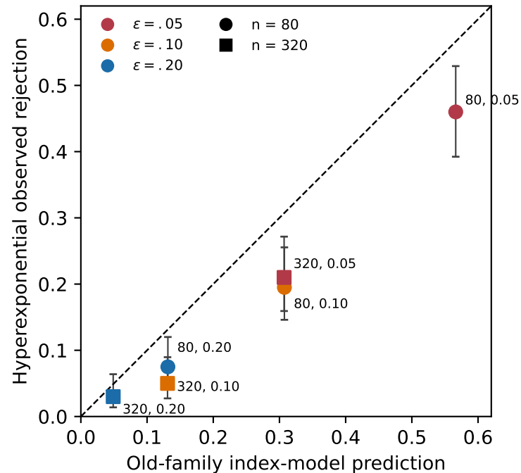
B. Prospective fifth-family residual (all predictions lie above observed rates)
