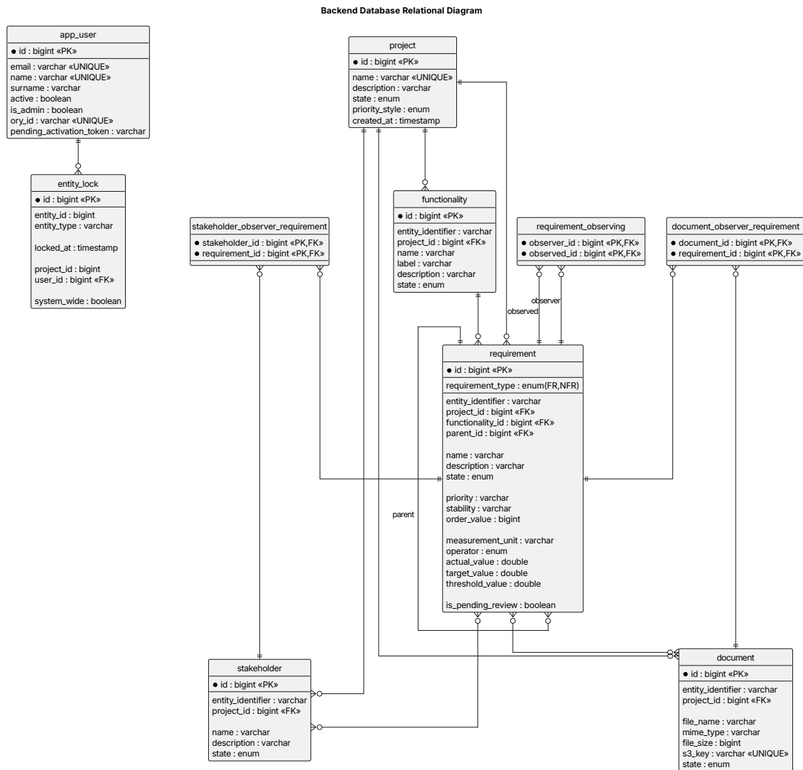
Figure 16: Relational database schema
