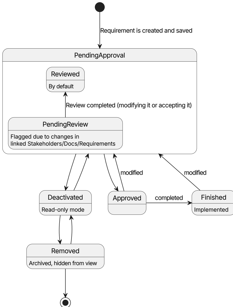
Figure 2: Requirement entity's state diagram
